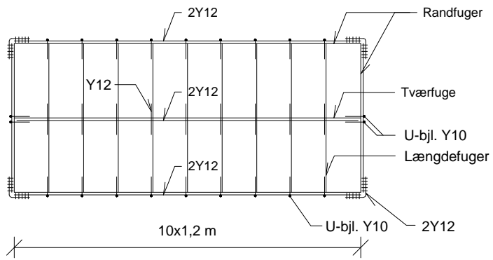
Figur 7.3.1/1 Fugearmeringsplan
